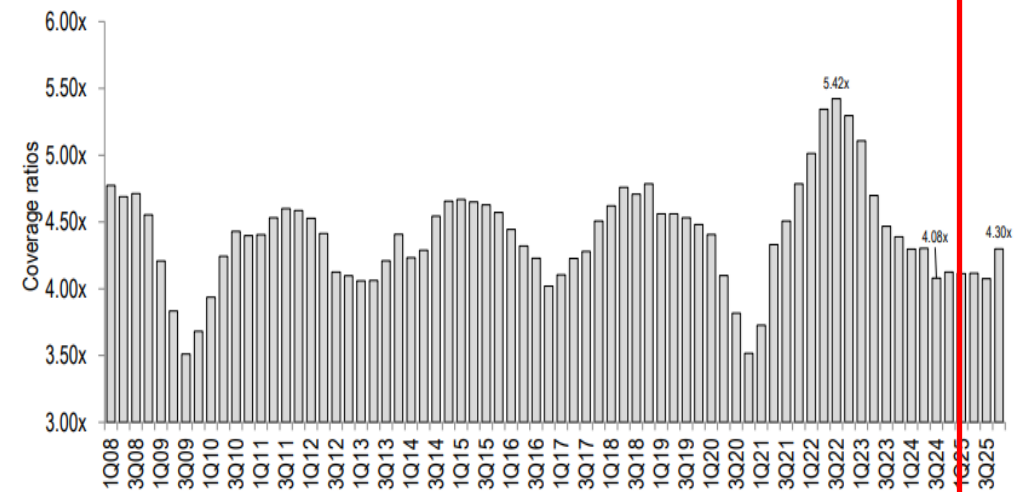
Coverage ratios for HY companies were higher in 4Q
